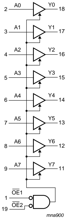
Fig 2. Functional diagram
