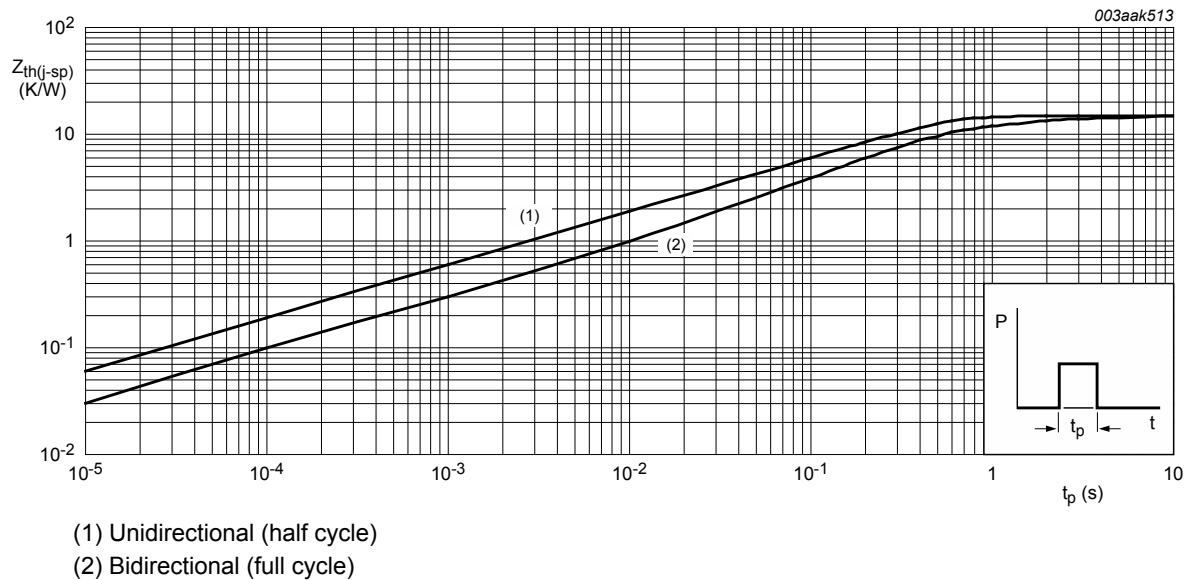
Fig. 6. Transient thermal impedance from junction to solder point as a function of pulse width
