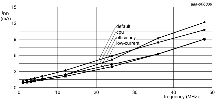
Fig 34. CoreMark current consumption for different power modes using external clock
