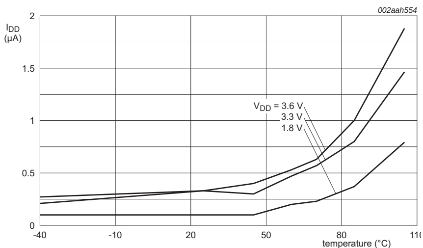
Fig 32. Deep power-down mode: Typical supply current I_{DD} versus temperature for different supply voltages V_{DD} (for LPC111xXL)
