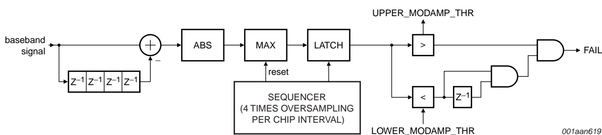
Fig 29. Block diagram of the modulation amplitude classification
