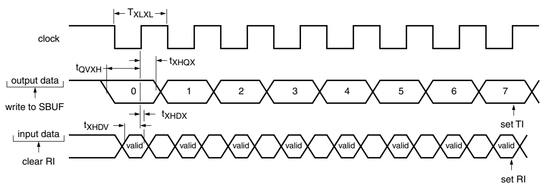
Fig 39. Shift register mode timing
