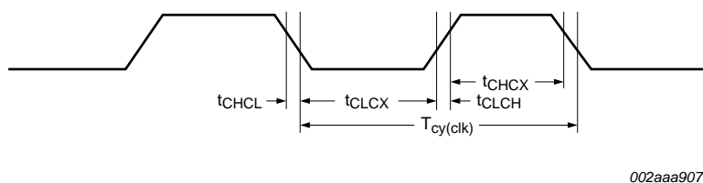
Fig 32. External clock timing (with an amplitude of at least V_{i(RMS)} = 200 mV)
