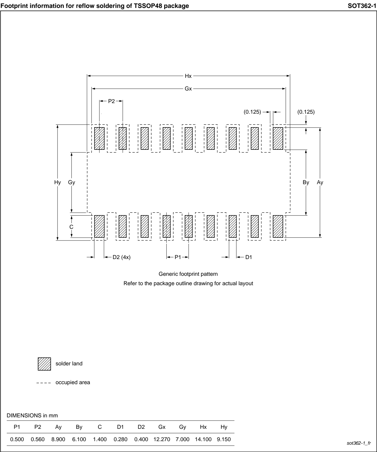
Fig 31. Footprint information for reflow soldering of SOT362-1 (TSSOP48) of PCA85162T
