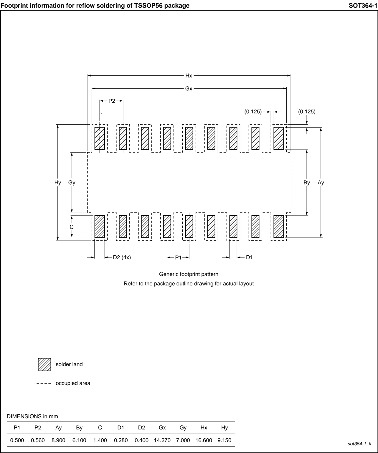
Fig 34. Footprint information for reflow soldering of SOT364-1 (TSSOP56) of PCA85176T
