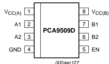
Fig 3. Pin configuration for SO8
