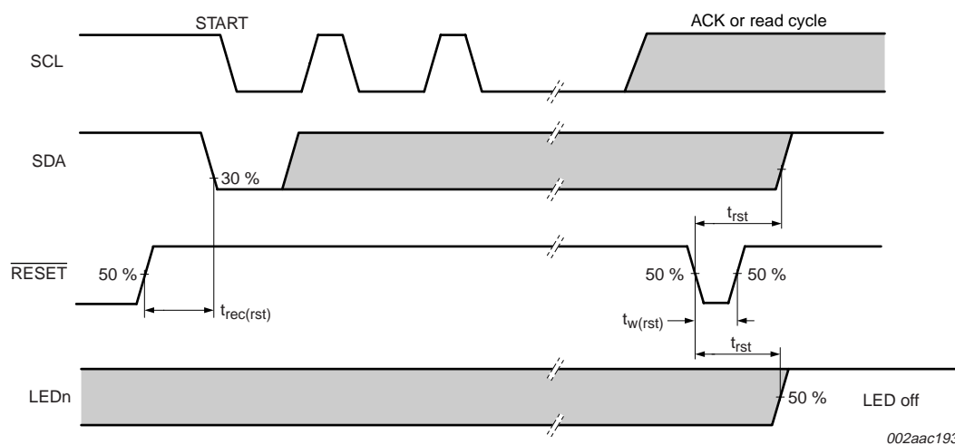
Fig 18. Definition of \overline{\text{RESET}} timing
