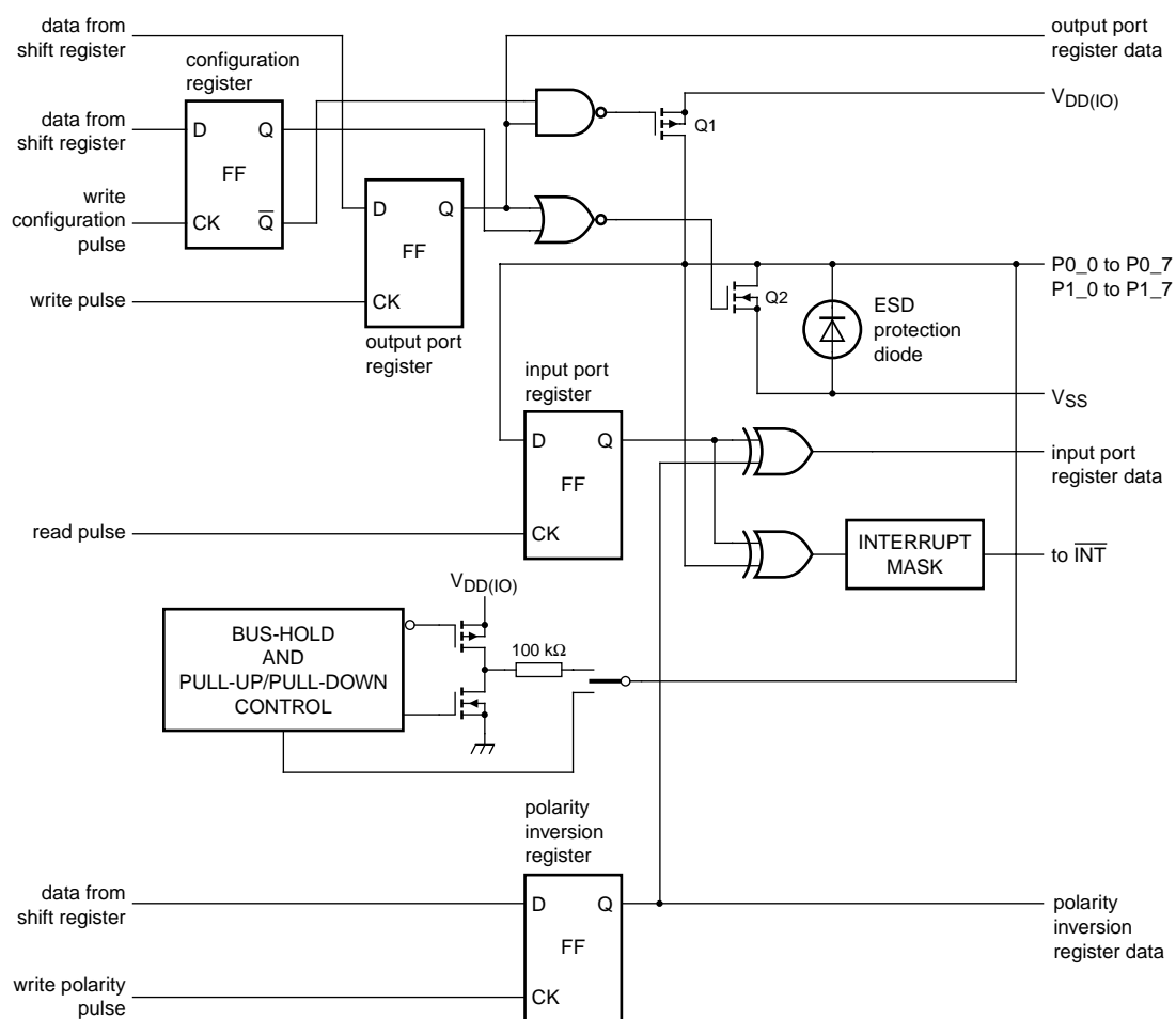
Fig 2. Simplified schematic of the I/Os (P0_0 to P0_7, P1_0 to P1_7)
