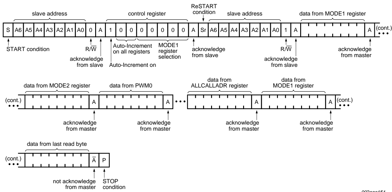
Fig 15. Read all registers using the Auto-Increment feature
