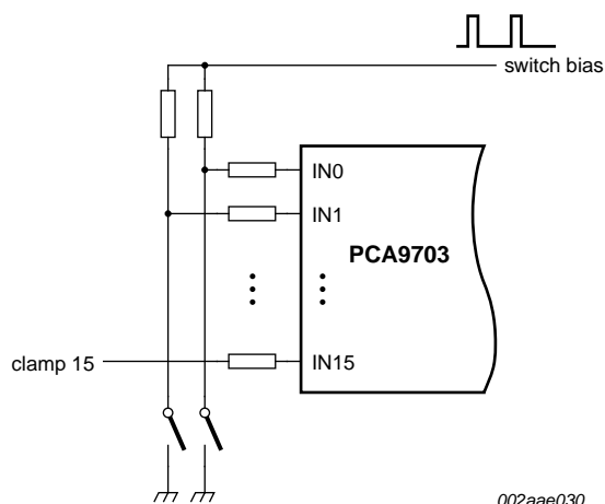
Fig 11. Clamp 15 (ignition) detection
