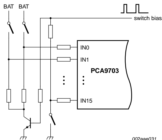
Fig 12. Switches to battery and ground with cyclic biasing
