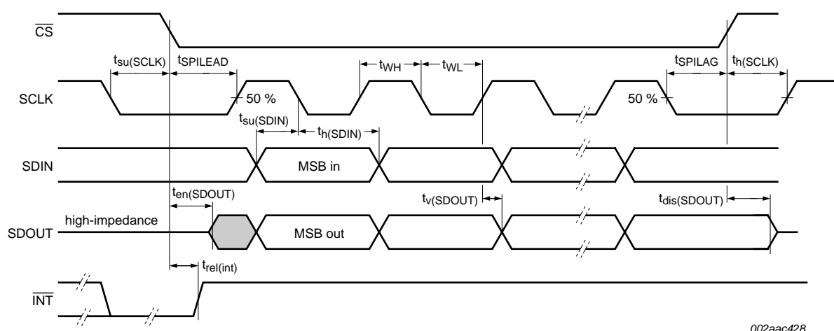
Fig 13. Timing diagram
