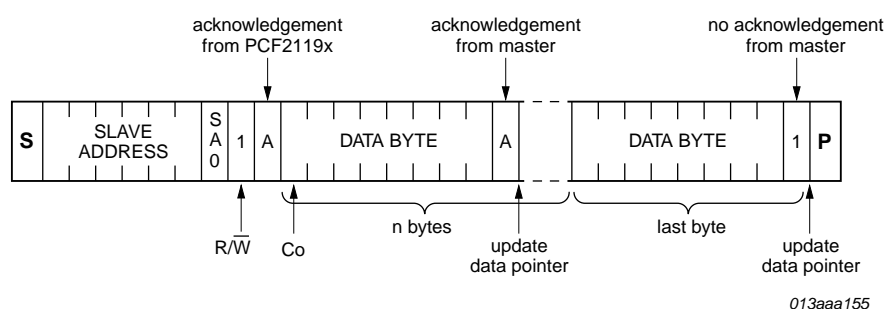
Fig 33. Master reads slave immediately after first byte; read mode (RS previously defined)
