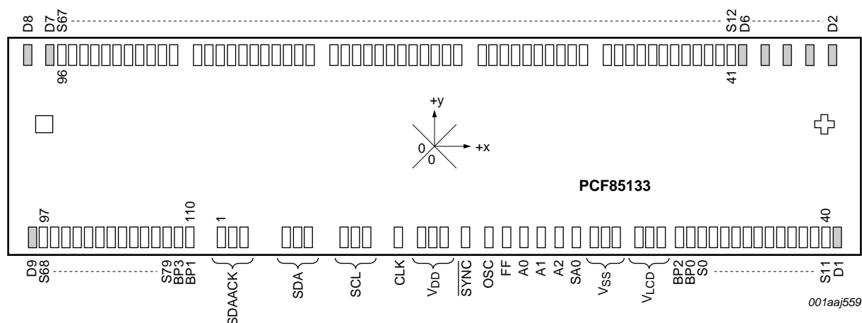
Fig 2. Pin configuration for PCF85133
