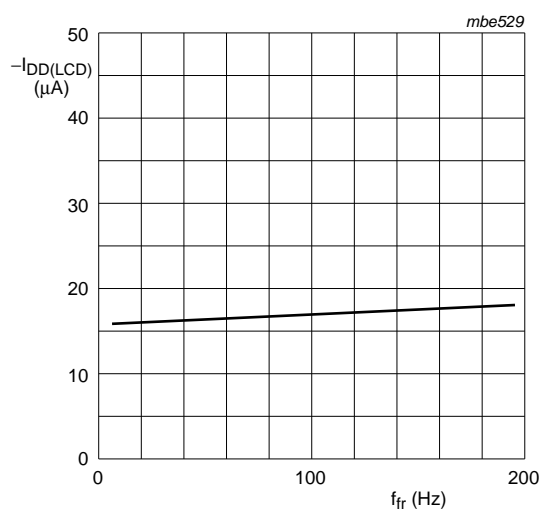
Fig 23. I_{DD(LCD)} as a function of f_{fr}
