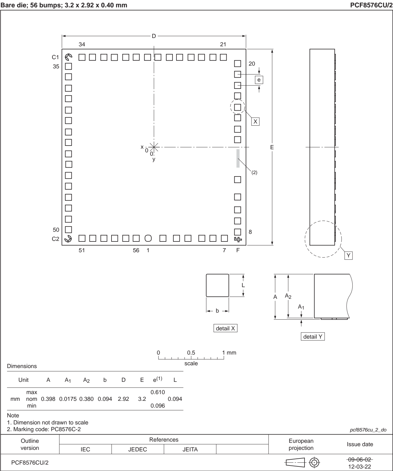
Fig 36. Bare die outline of PCF8576CU/2/F2
