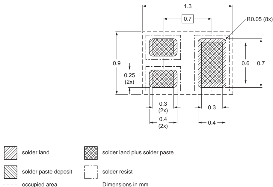
Fig 11. Reflow soldering footprint for SOT883B (DFN1006B-3)
