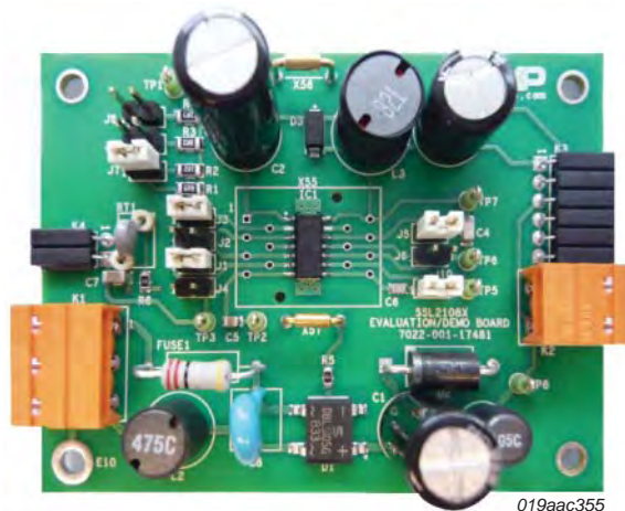
b. Top view: SSL21082 (SO12).
