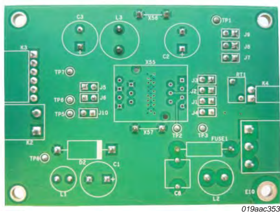
Fig 15. SSL21081 and SSL21082 evaluation board photographs
