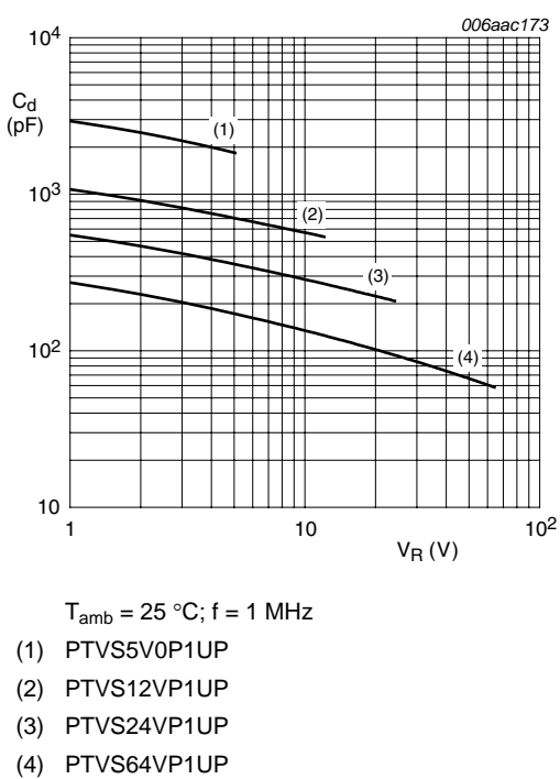
Fig 4. Diode capacitance as a function of reverse voltage; typical values
