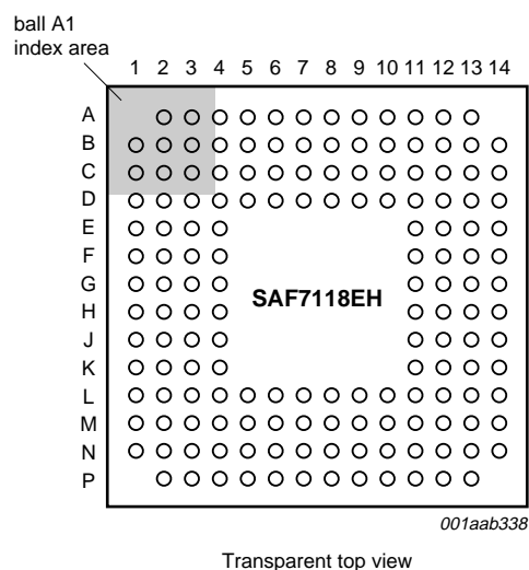
Fig 3. Pin configuration (HBGA156)
