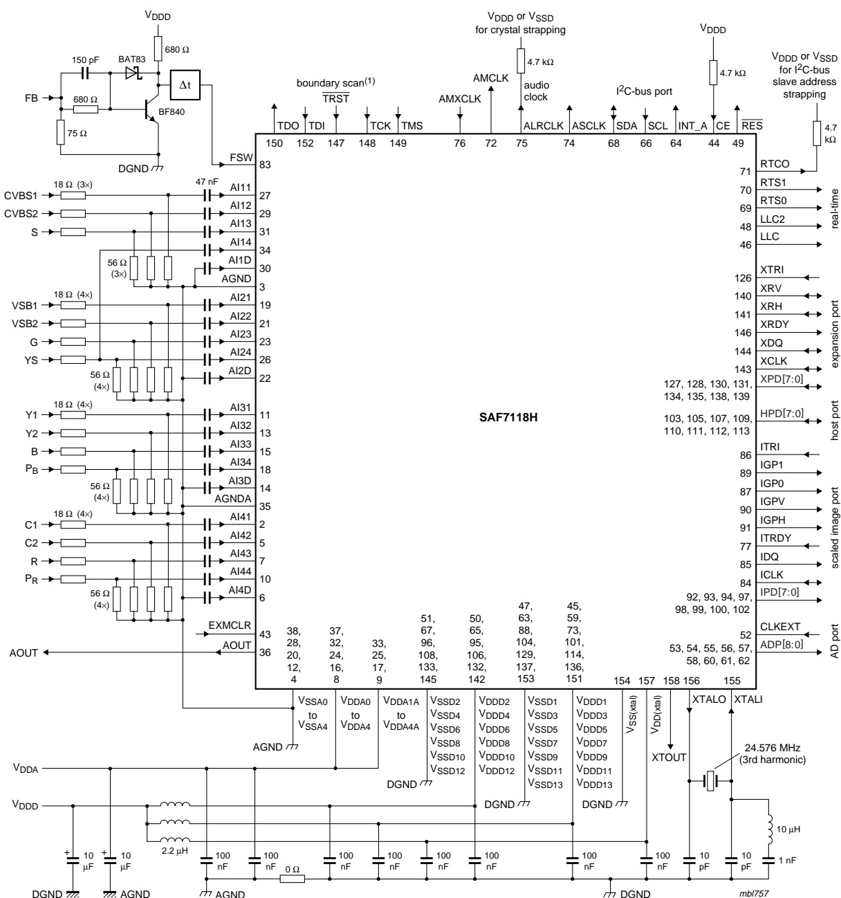
Fig 93. Application example with 24.576 MHz crystal (QFP160 package)
