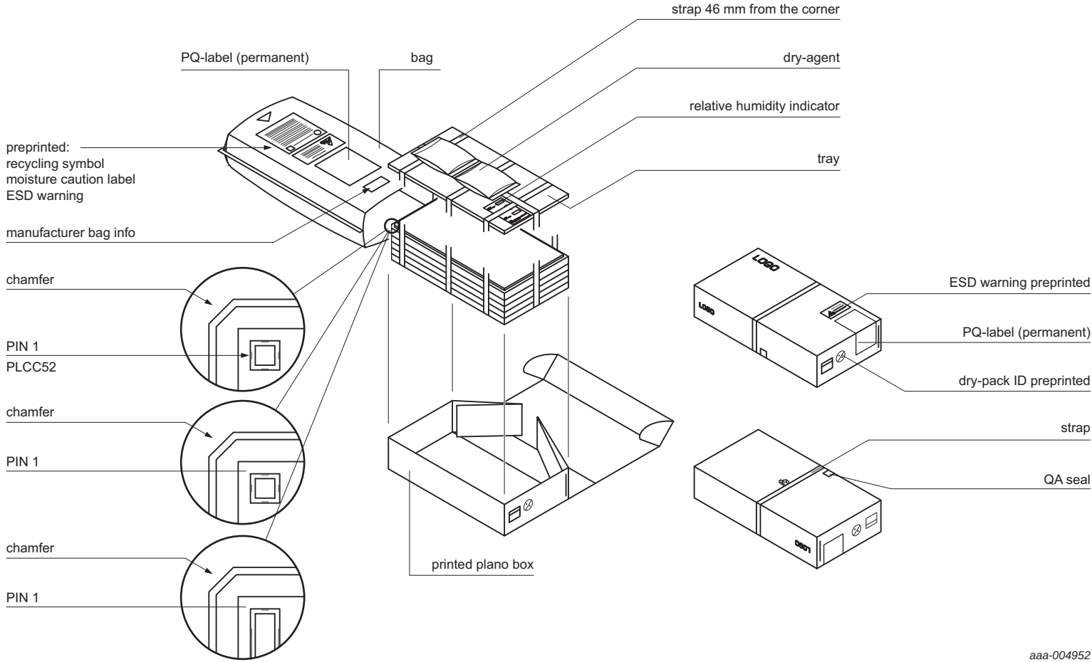
Fig 33. Packing information 5 tray
