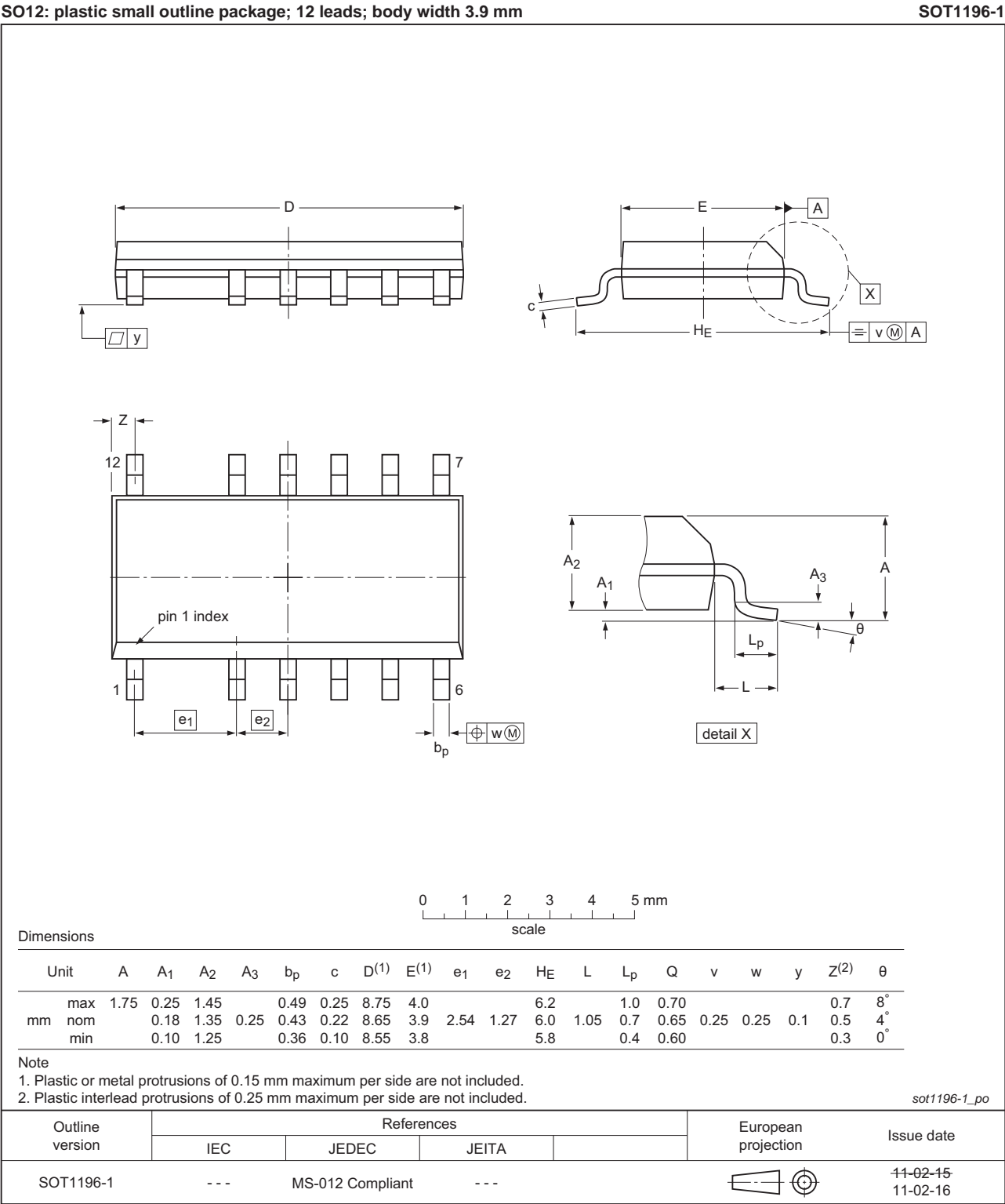
Fig 7. Package outline SOT1196-1 (SO12)
