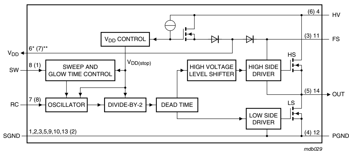
Fig 1. Block diagram
