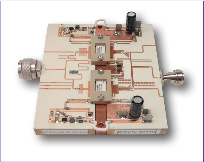
Asymmetrical Doherty demoboard using BLF7G24LS-100 as the main amplifier and BLF7G24LS-140 as the peak amplifier
