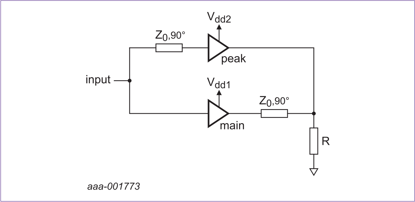
Doherty block diagram – as used by BLF7G24L(S) family
