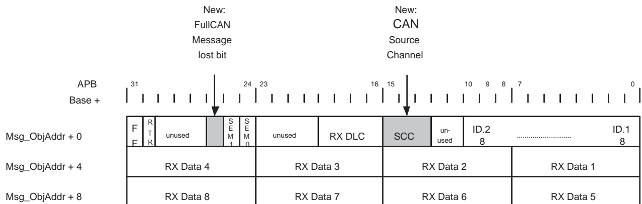
Fig 64. FullCAN message object layout
