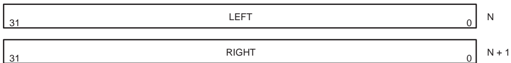
Fig 113. FIFO contents for various I2S modes
