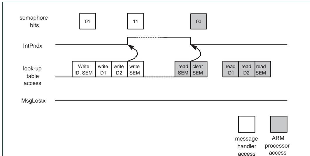
Fig 65. Normal case, no messages lost
