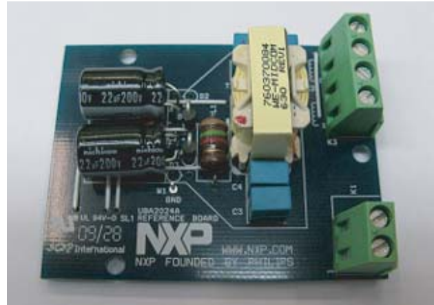
Fig 4. UBA2024AT 120 V (AC) mains demo board
