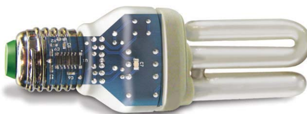
Fig 8. Proposed board placement in a lamp for the UBA2024AT to reduce radiated heat to the IC
