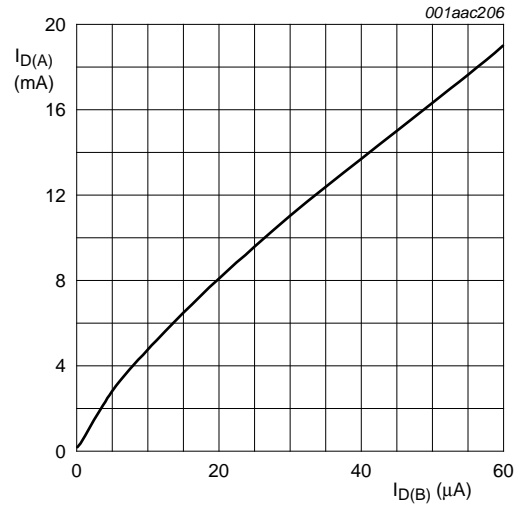
V_{DS(A)} = 5 \text{ V} ; V_{G2-S} = 4 \text{ V} ; V_{DS(B)} = 5 \text{ V} ; V_{G1-S(B)} = 0 \text{ V} ; T_j = 25 \text{ }^\circ\text{C} . I_{D(B)} = internal G1 current = current in pin drain (B) if MOSFET (B) is switched off.
