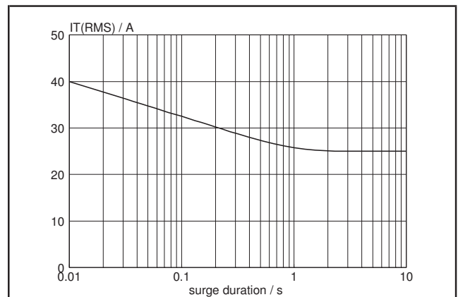
Fig.5. Maximum permissible repetitive rms on-state current I_{T(RMS)} , versus surge duration, for sinusoidal currents, f = 50 Hz; T_{mb} \leq 91^\circ\text{C} .
