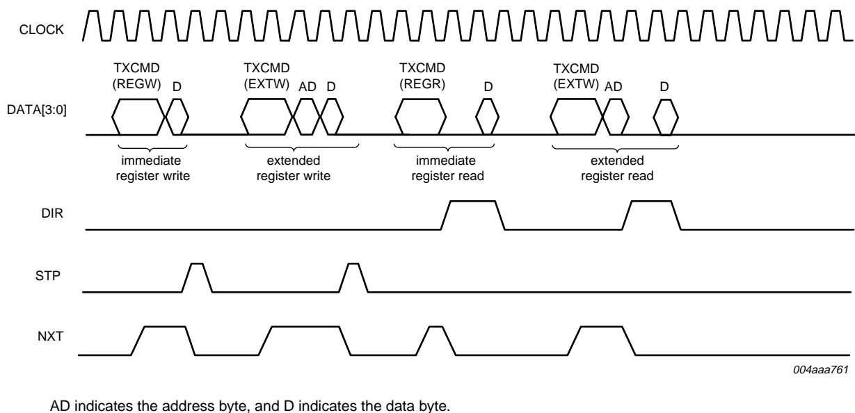
Fig 10. Example of register write, register read, extended register write and extended register read
