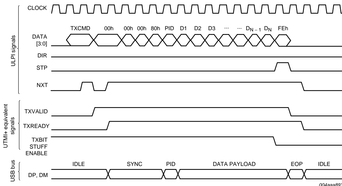
Fig 19. Transmitting USB packets without automatic SYNC and EOP generation
