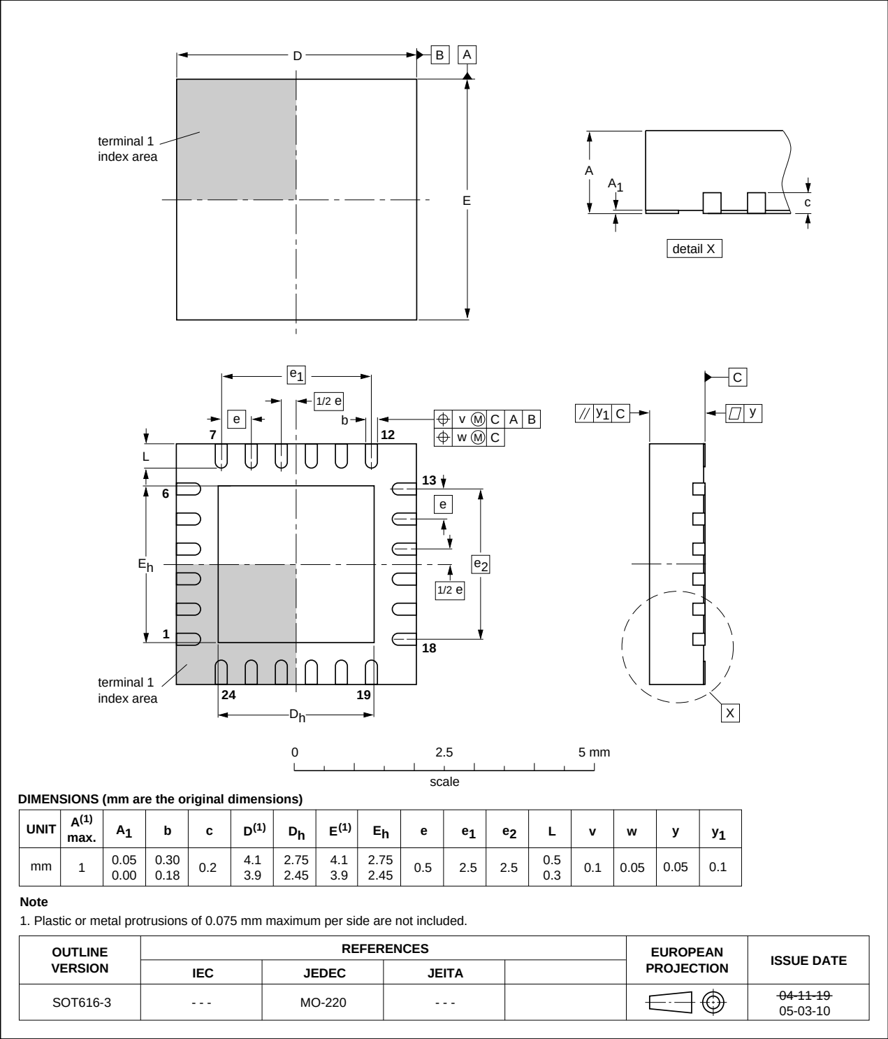
Fig 58. Package outline SOT616-3 (HVQFN24)
