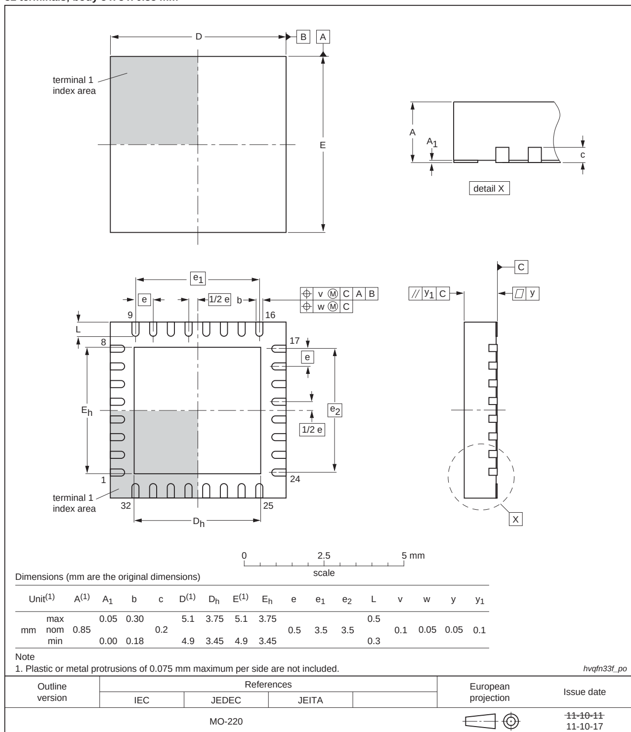
Fig 55. Package outline (HVQFN33 5x5)
