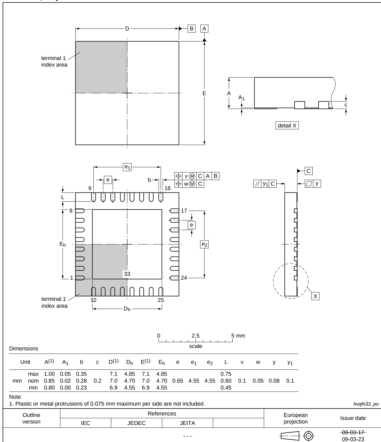
Fig 56. Package outline (HVQFN33 7x7)
