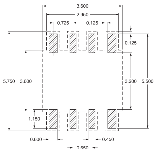
Fig 23. PCB footprint for SOT505-1 (TSSOP8); reflow soldering
