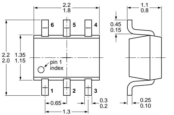
Fig 11. Package outline PUMH1 (SOT363)
