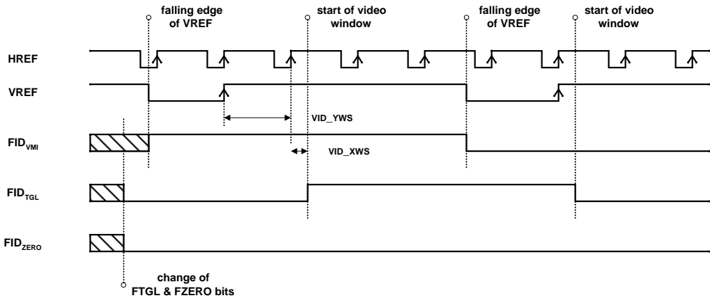
Figure 10: Field Identifier Timing
