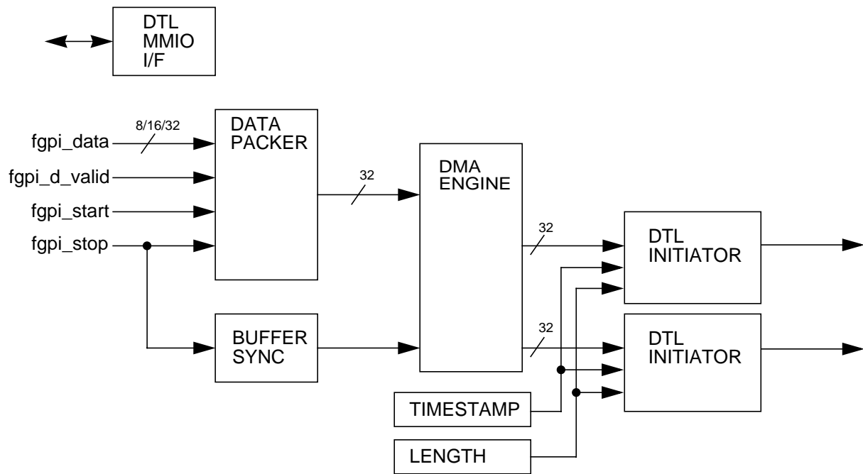
Figure 2: FGPI Module Block Diagram
