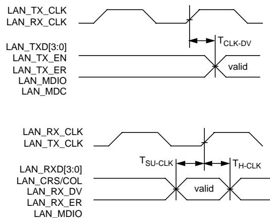
Figure 14: LAN 10/100 I/O Timing in MII Mode
