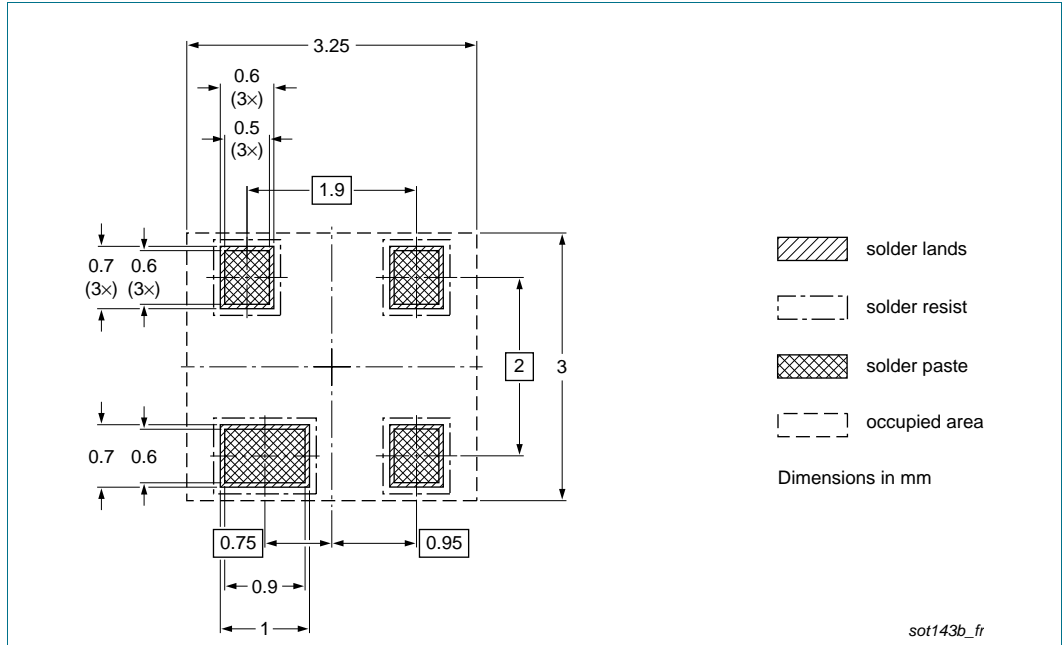
Fig 6. Reflow soldering footprint SOT143B
