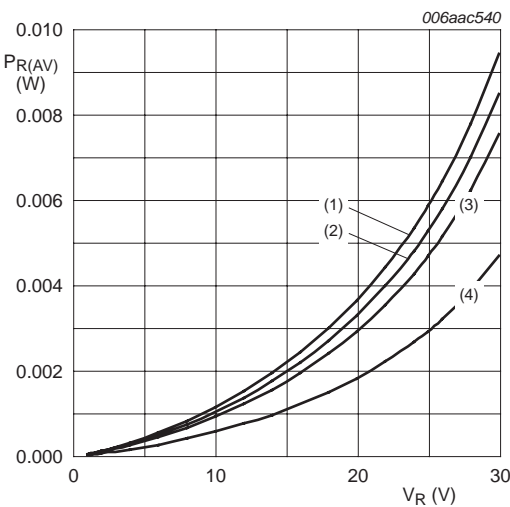
T_j = 125\text{ }^{\circ}\text{C} (1) \delta = 1 ; DC (2) \delta = 0.9 ; f = 20\text{ kHz} (3) \delta = 0.8 ; f = 20\text{ kHz} (4) \delta = 0.5 ; f = 20\text{ kHz}
