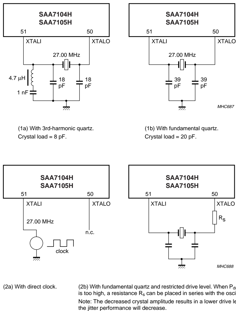
Fig.18 Oscillator application.
