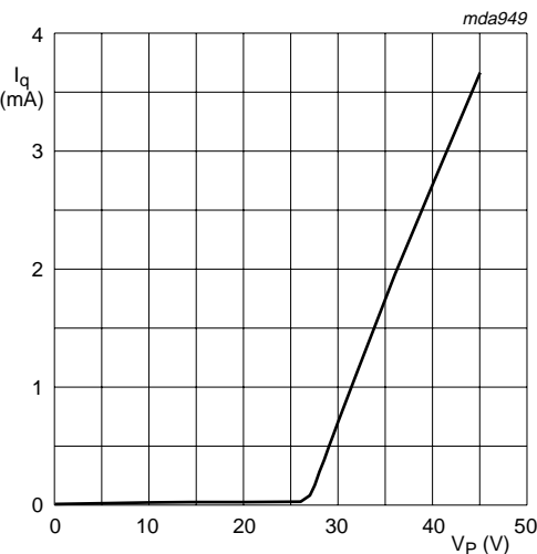
Fig 6. Quiescent current increase at high supply voltage
