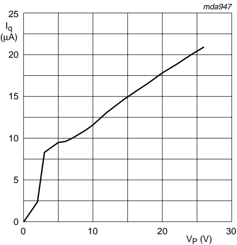
Fig 4. Quiescent current as a function of the supply voltage
