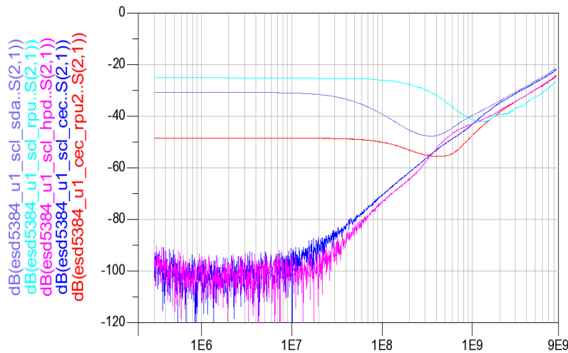
Figure 2. Crosstalk Measurements
