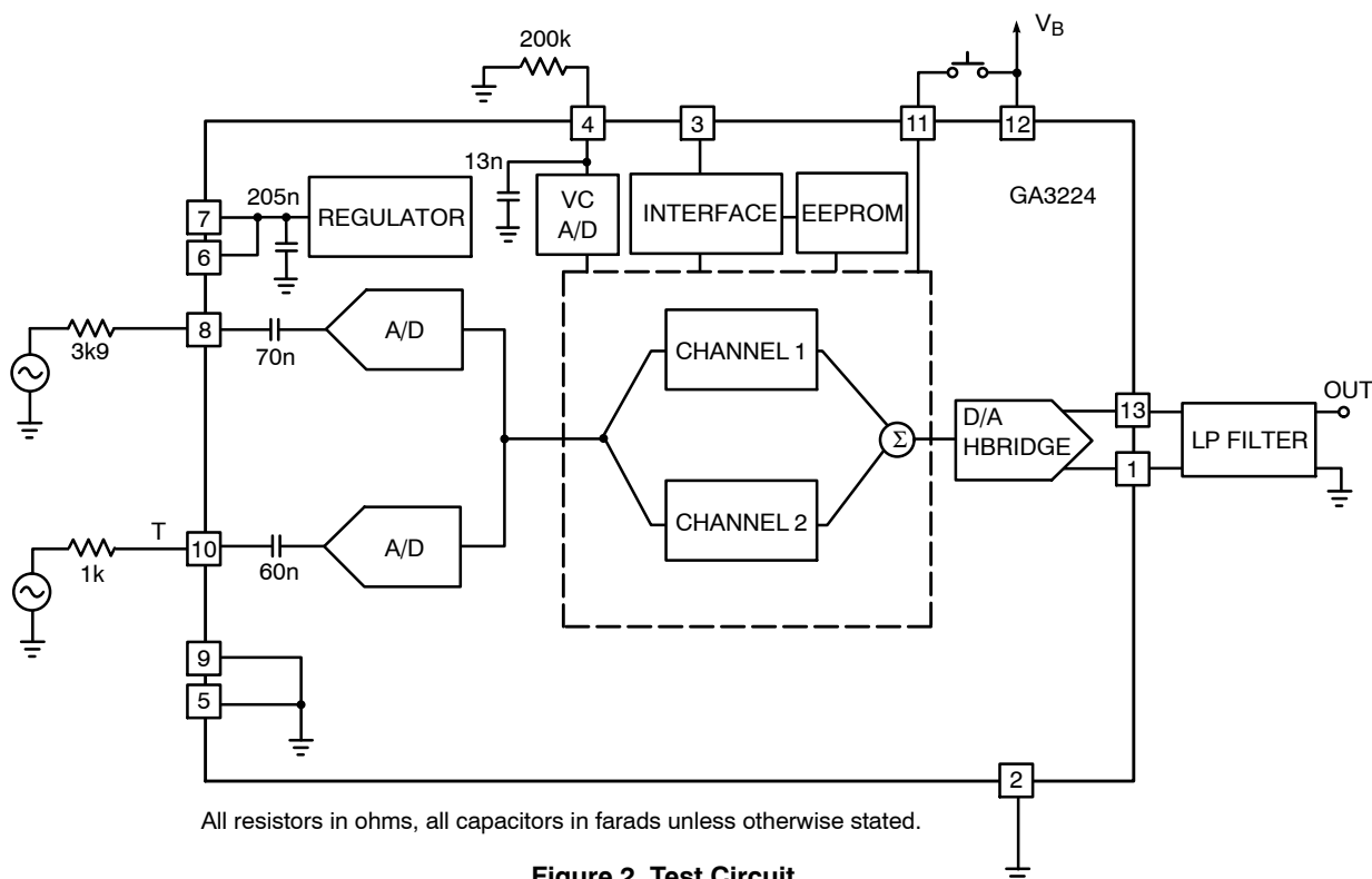
Figure 2. Test Circuit
