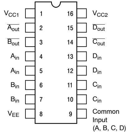
Figure 2. Pin Assignment
