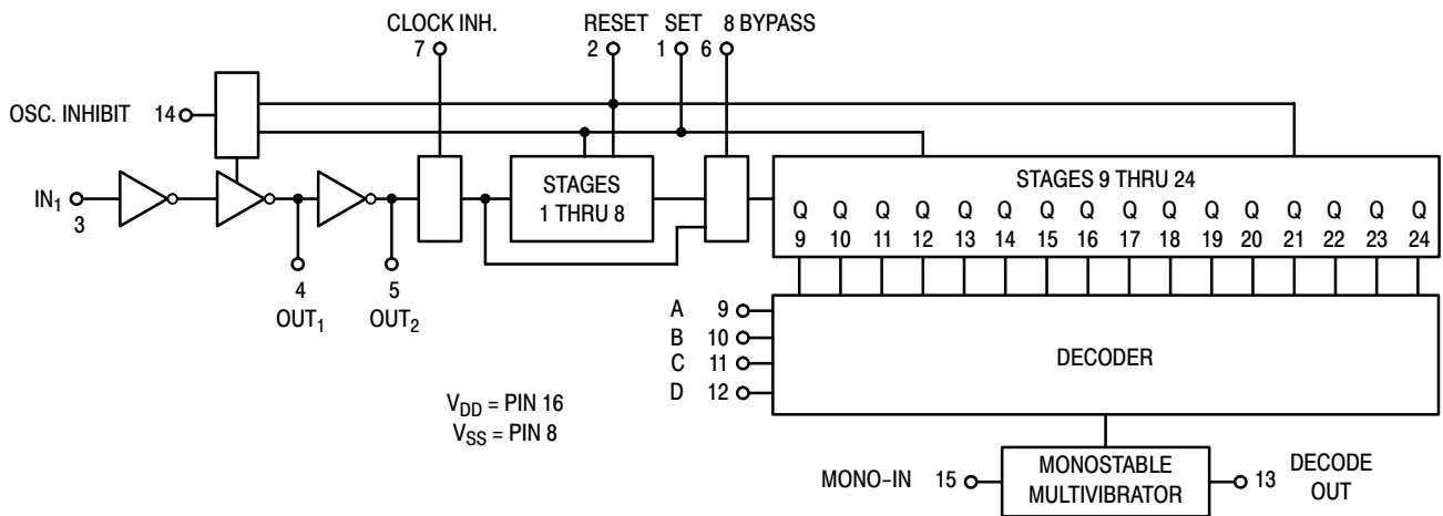
Figure 2. Block Diagram
