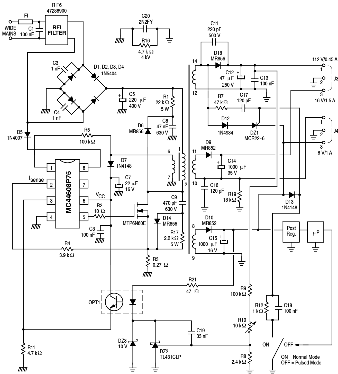
Figure 18. Typical Application
