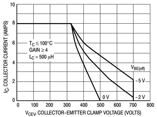
Figure 7. Maximum Reverse Bias Switching Safe Operating Area
