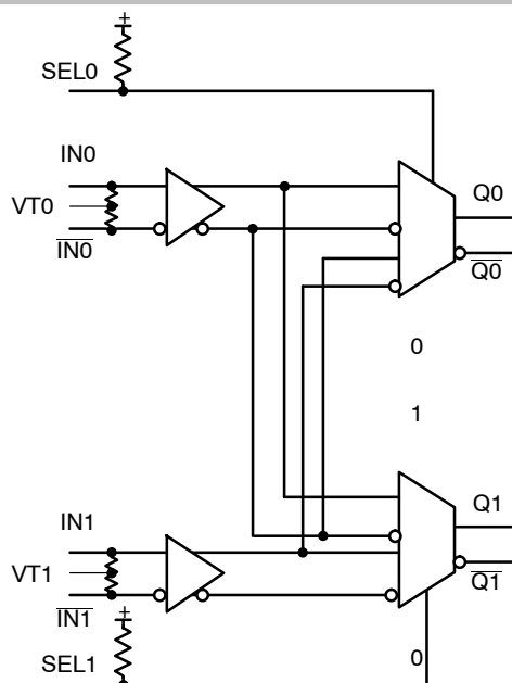
Figure 1. Logic Diagram 1
