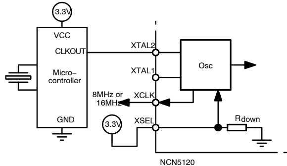
Figure 19. External Clock Generator
