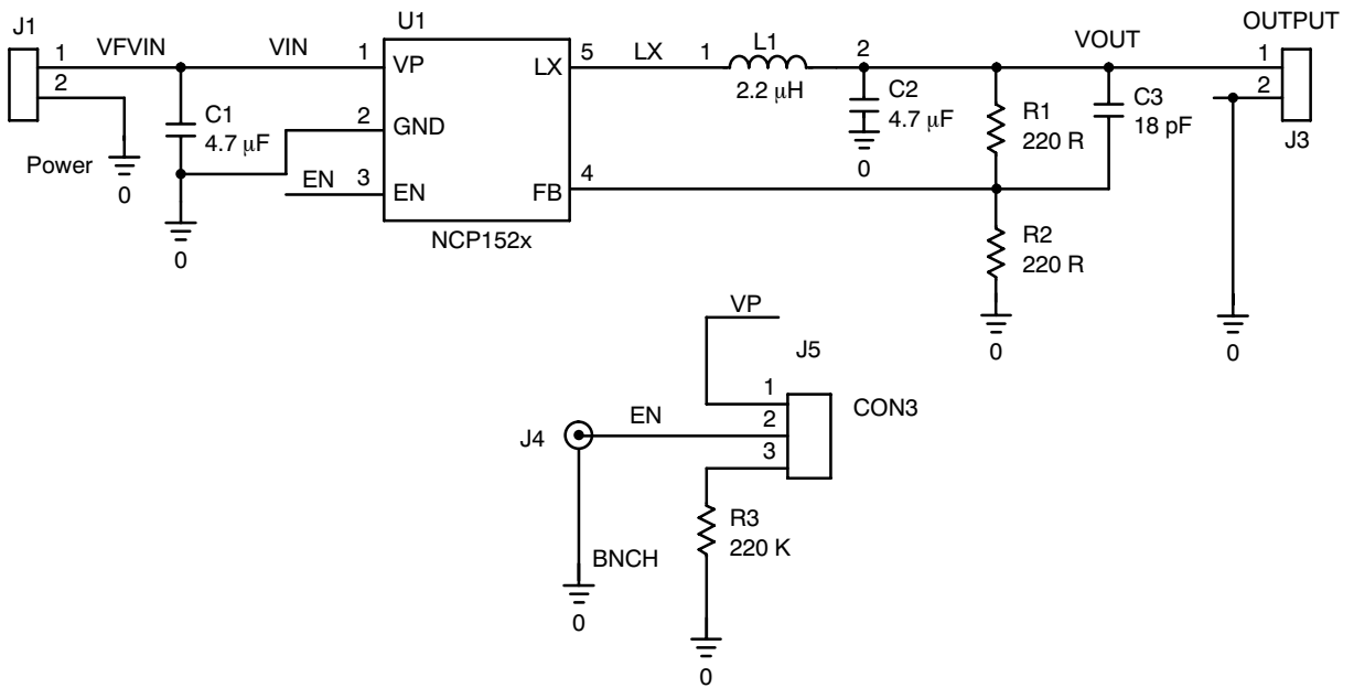
Figure 27. Schematics
