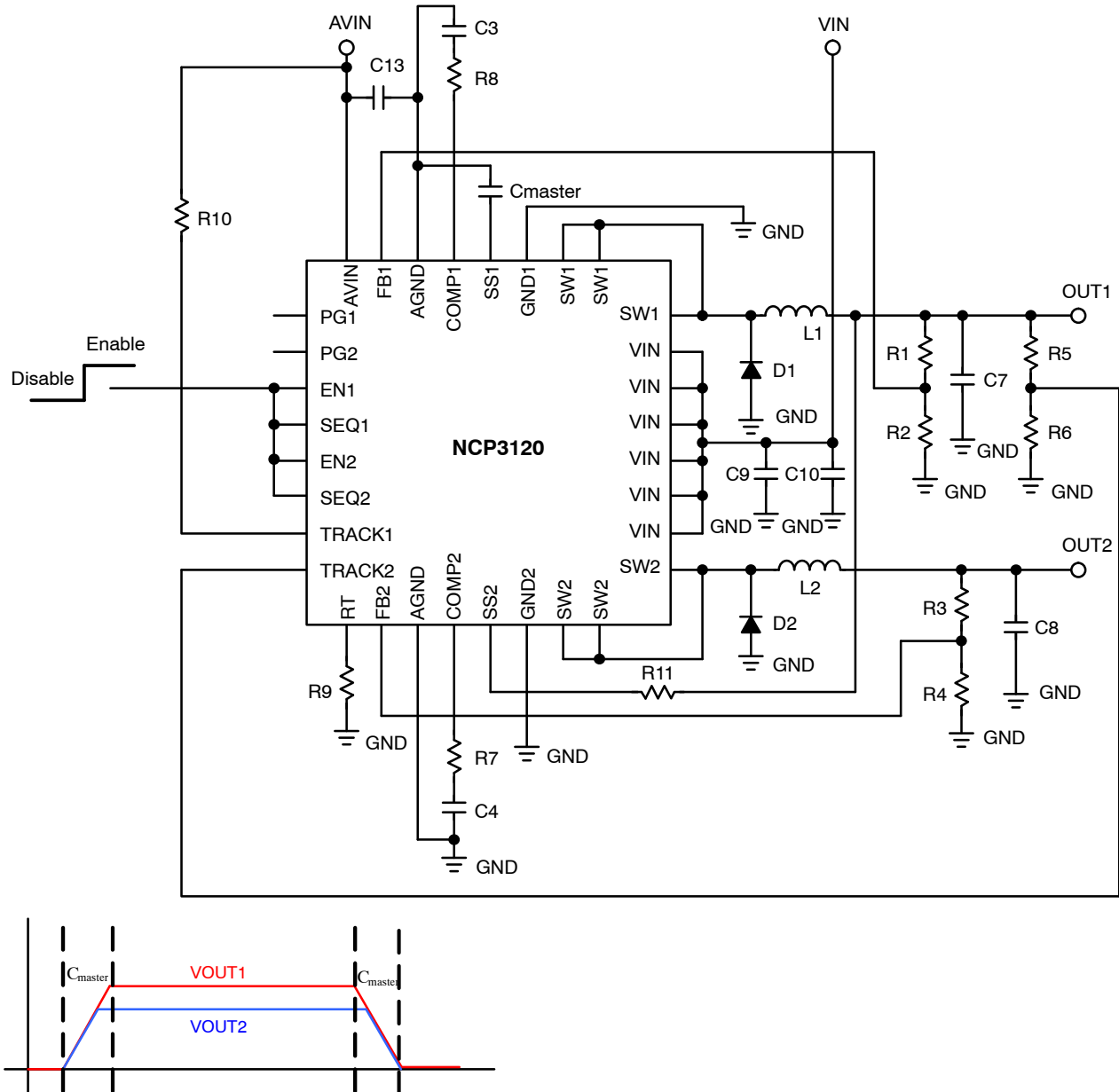
Figure 51. Tracking Configuration
