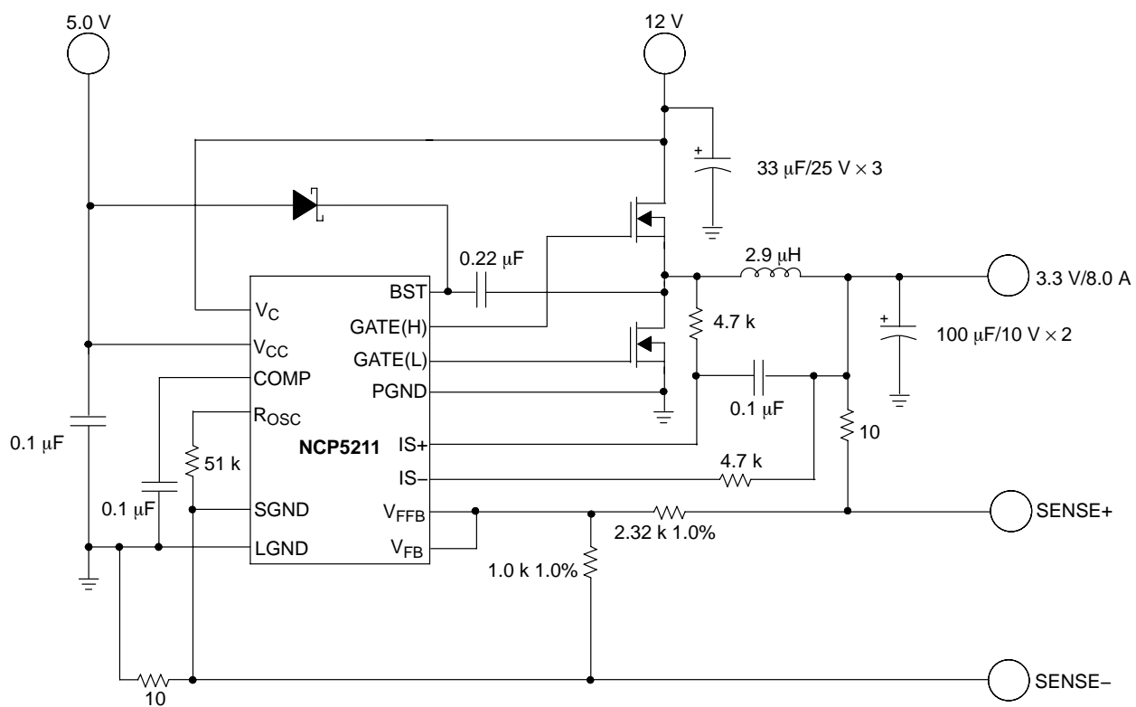
Figure 10. Additional Application Diagram, 12 V to 5.0 V Bias to 3.3 V/8.0 A Converter with Differential Remote Sense
