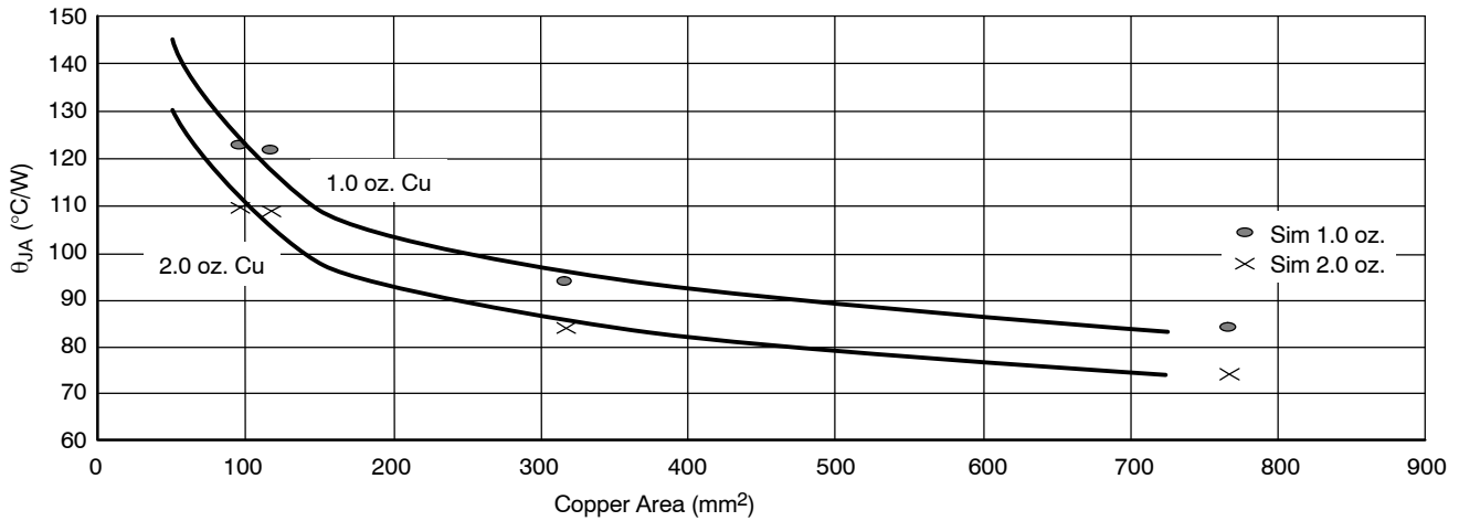
Figure 19. SOIC-14, \theta_{\text{JA}} as a Function of the Pad Copper Area Including Traces, Board Material
